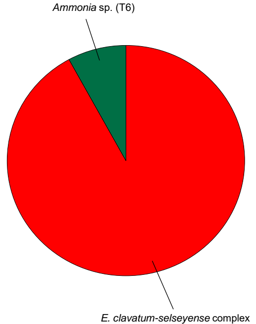
Hanö Bay, Baltic Sea (Total (live+dead) C-Ha-1a)
