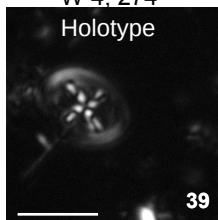
C. fahudensis sp. nov. W-3, 152
