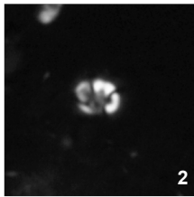
cf. Calcu. additus W-4, 307.8
