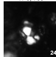
Oct. multiplus W-5, 755
