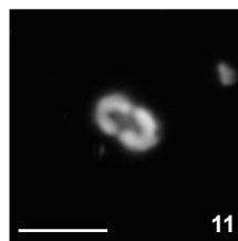
Bif. mchanae W-4, 1295.4
