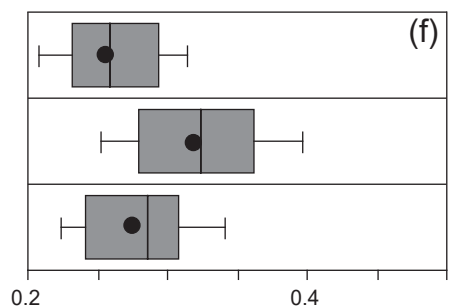
Central area Width / Coccolith Width ratio
