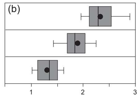
Central area Width [ \mu\text{m} ]
