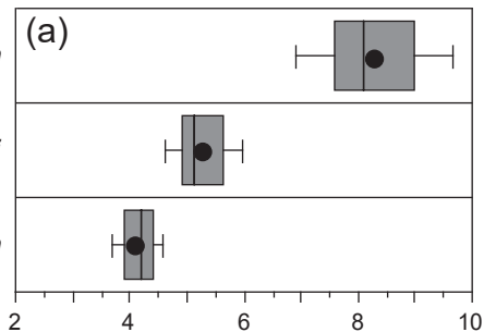
Coccolith Width [ \mu\text{m} ]
