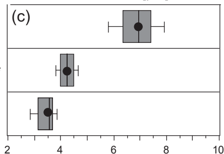
Central area Length / Coccolith Length ratio
