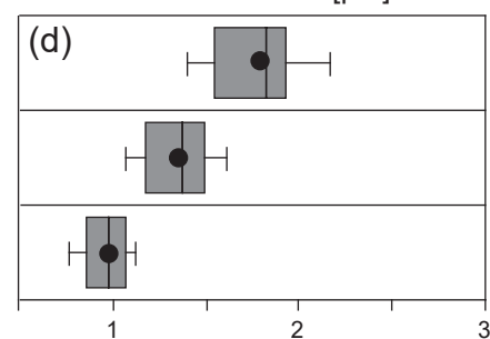
Central area Width / Coccolith Width ratio
