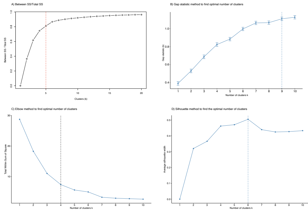
Fig. S2. Various methods to define the optimal clustering for dinocyst data in wsi_100.
