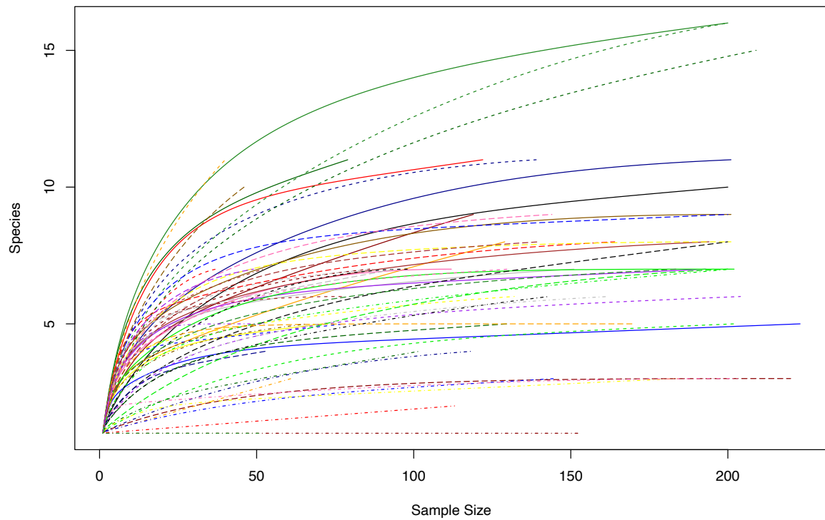
Figure S1. Rarefaction on dinocyst counts of the new samples.
