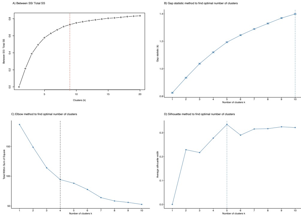
Fig. S3 Various methods to determine the optimal clustering of the dinocyst data in sh_655.
