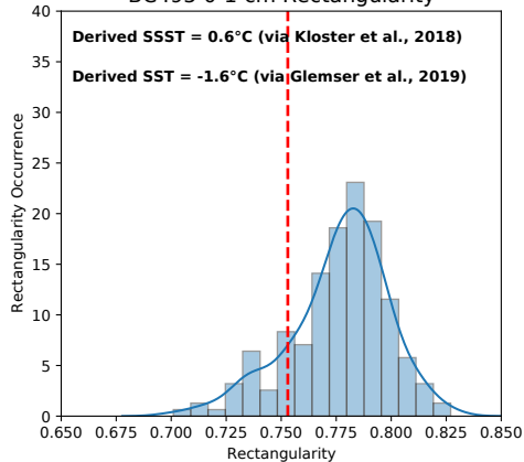
BC495 0-1 cm Rectangularity
