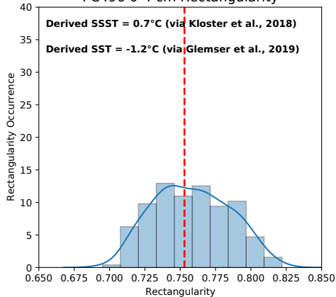
PC496 0-4 cm Rectangularity
