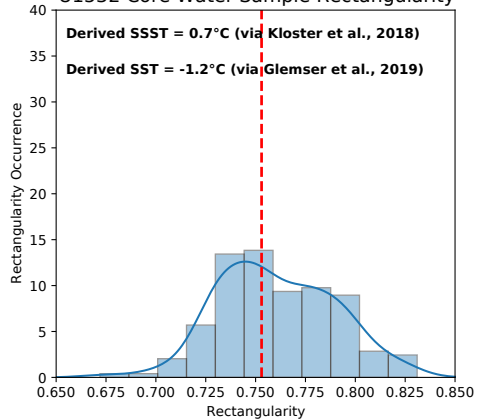
U1532 Core Water Sample Rectangularity
