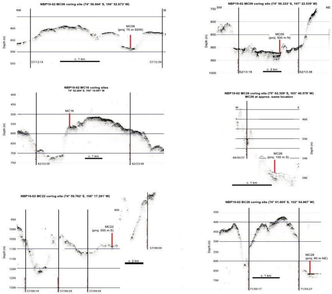
Figure S1. Sections of Knudsen acoustic sub-bottom profiles across/near the studied core sites. The red line indicates the (projected) location of a core site.
